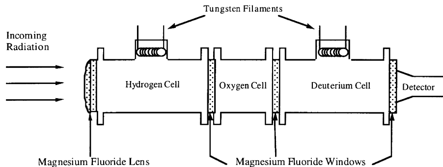
Figure 9. Conceptual diagram of the Cassini Hydrogen Deuterium Absorption Cell (HDAC). The tungsten filaments dissociate molecular hydrogen and deuterium inside the cells. The dissociated atoms resonantly absorb hydrogen and deuterium Lyman- \alpha . Cycling the filament currents in both the hydrogen and deuterium cells gives a direct measurement of the hydrogen and deuterium Lyman- \alpha intensities.
