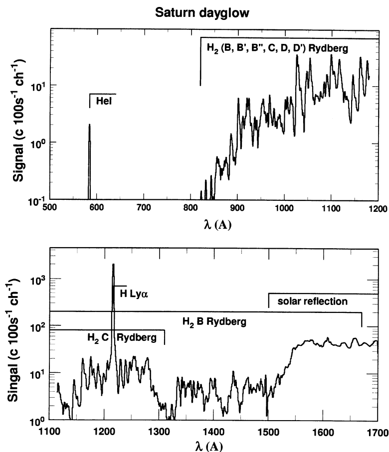
Figure 22. Model synthesis of Saturn dayglow spectra in the UVIS EUV and FUV channels showing soft-electron excited H 2 and H. The long wavelength region is dominated by the reflection of solar radiation. A brightness of 1.0 kR for the H 2 bands is assumed, matching the value obtained by the Voyager UVS experiment.
