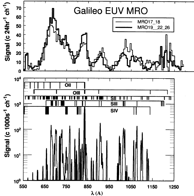
Figure 24. Comparison of modeled UVIS spectrum of Io plasma torus with Galileo observation. The predicted UVIS spectrum at 2.4 \text{ \AA} resolution obtains higher total signal counts in 1000 s than those obtained by the Galileo EUV instrument in 24 h, at a resolution of 40 \text{ \AA} .
